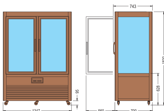
SALOON 1000 G•RG
