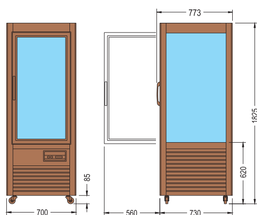
SALOON 500 R•G•Q
