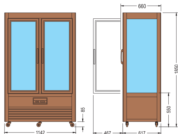
SALOON 700 Q•G•RG
