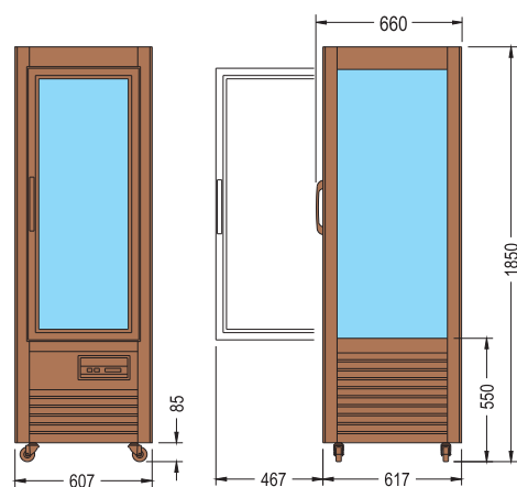
SALOON 350 R•G•Q
